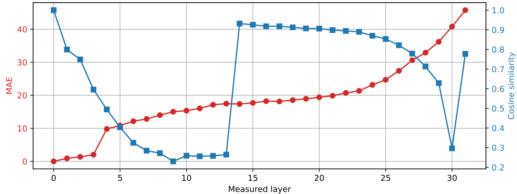
SmolLM2-360M | Prompt 4 Spared layer 16 | Hybrid vs unquantized
