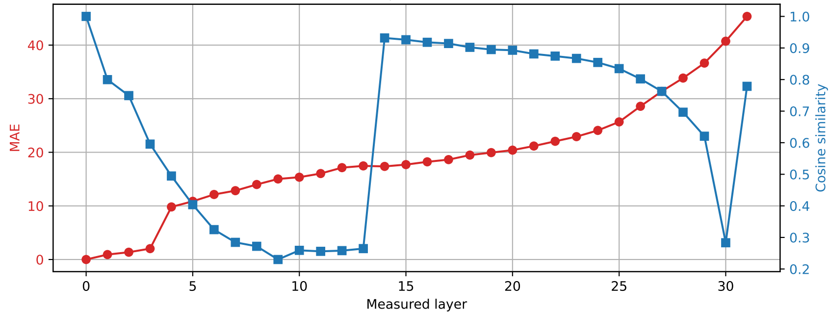
SmolLM2-360M | Prompt 4 Spared layer 23 | Hybrid vs unquantized
