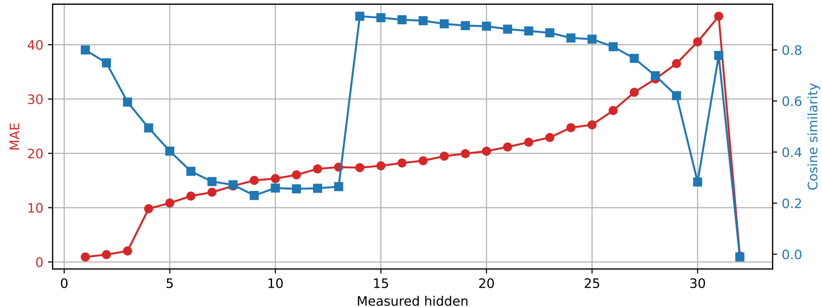
SmolLM2-360M | Prompt 4 Spared layer 24 | Unquantized vs hybrid
