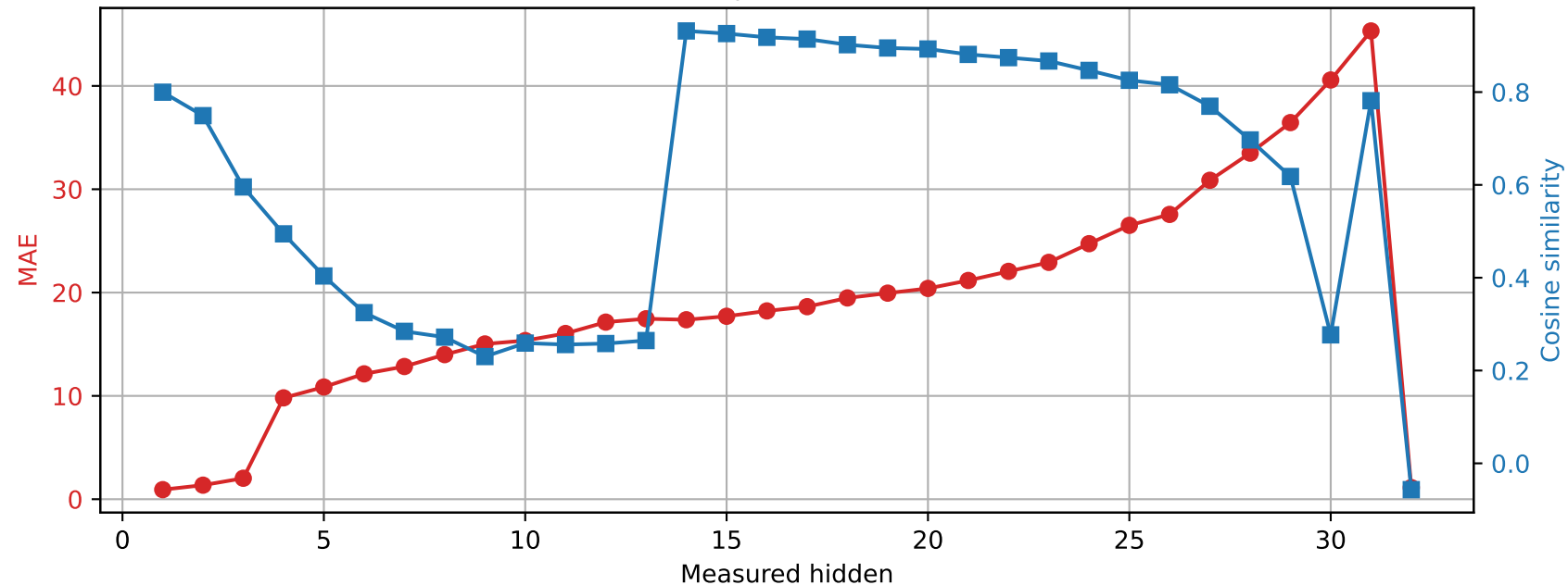
SmolLM2-360M | Prompt 4 Spared layer 25 | Unquantized vs hybrid
