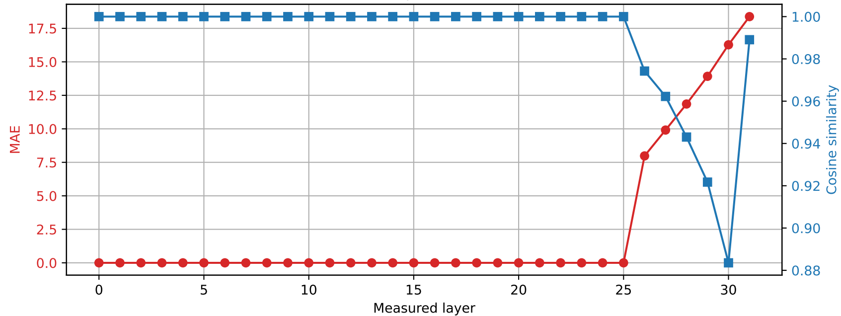
SmolLM2-360M | Prompt 4 Spared layer 25 | Hybrid vs quantized
