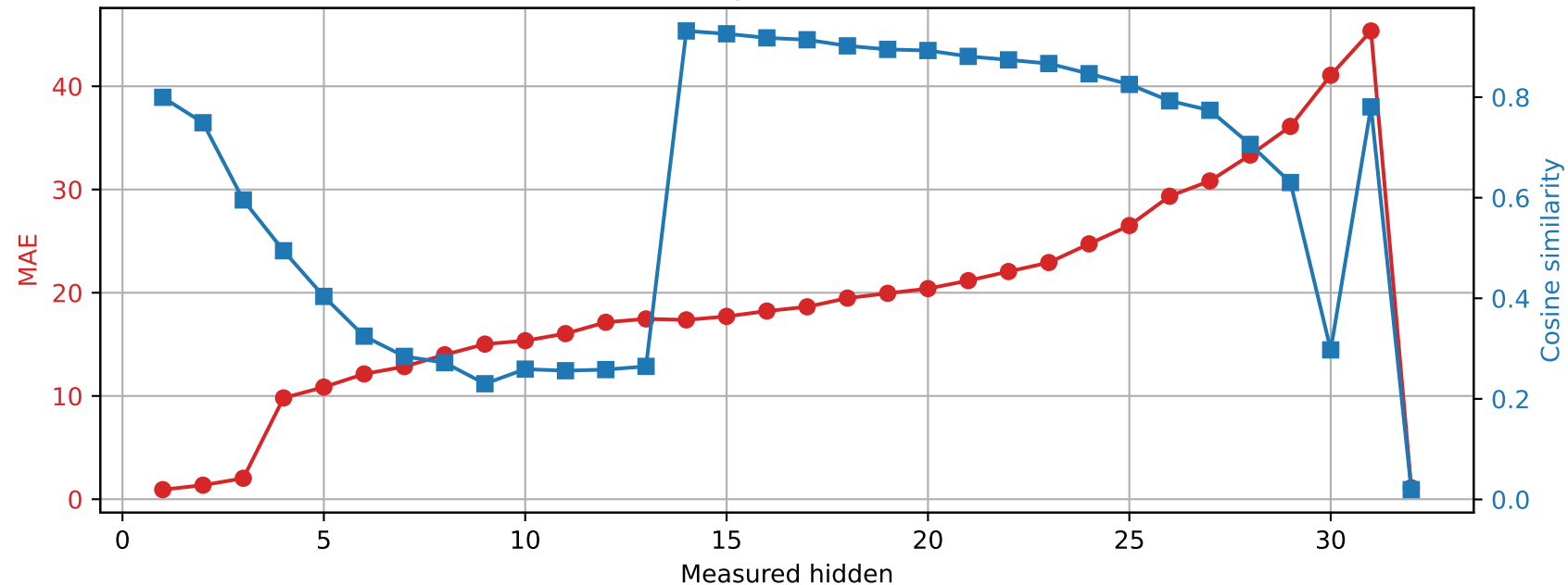
SmolLM2-360M | Prompt 4 Spared layer 26 | Unquantized vs hybrid
