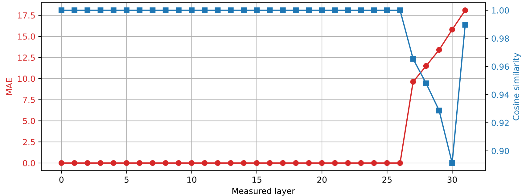
SmolLM2-360M | Prompt 4 Spared layer 26 | Hybrid vs quantized
