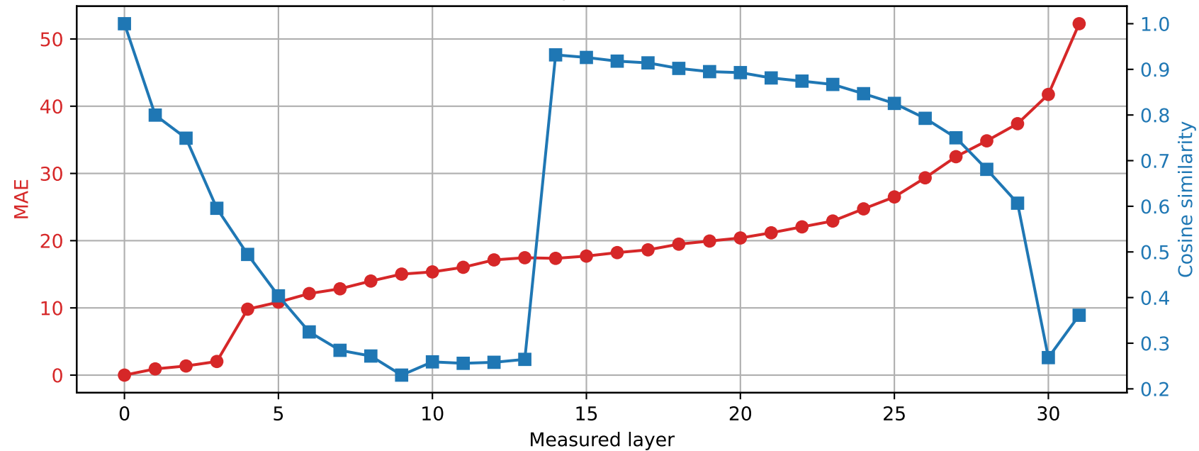
SmolLM2-360M | Prompt 4 Spared layer 30 | Hybrid vs unquantized
