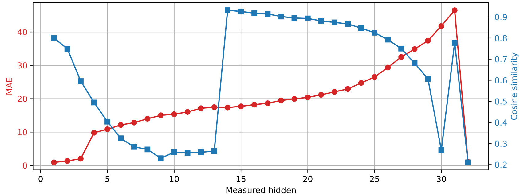
SmolLM2-360M | Prompt 4 Spared layer 31 | Unquantized vs hybrid
