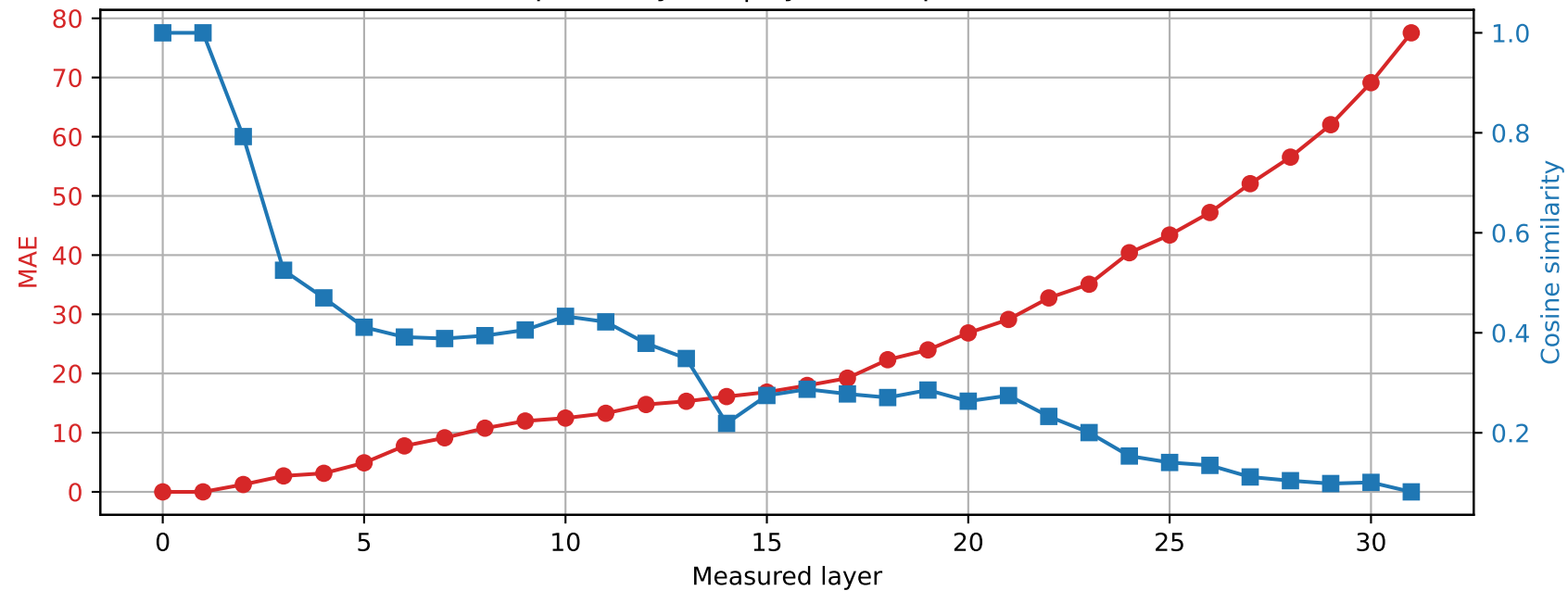
SmolLM2-360M | Prompt 0 Spared layer 1 | Hybrid vs quantized
