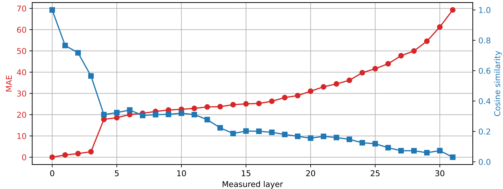
SmolLM2-360M | Prompt 0 Spared layer 4 | Hybrid vs unquantized
