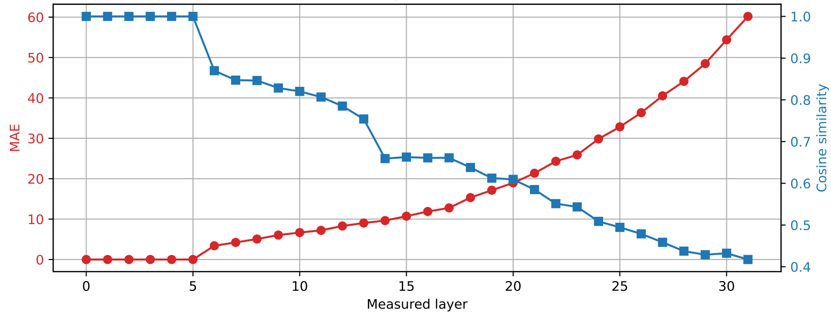
SmolLM2-360M | Prompt 0 Spared layer 5 | Hybrid vs quantized
