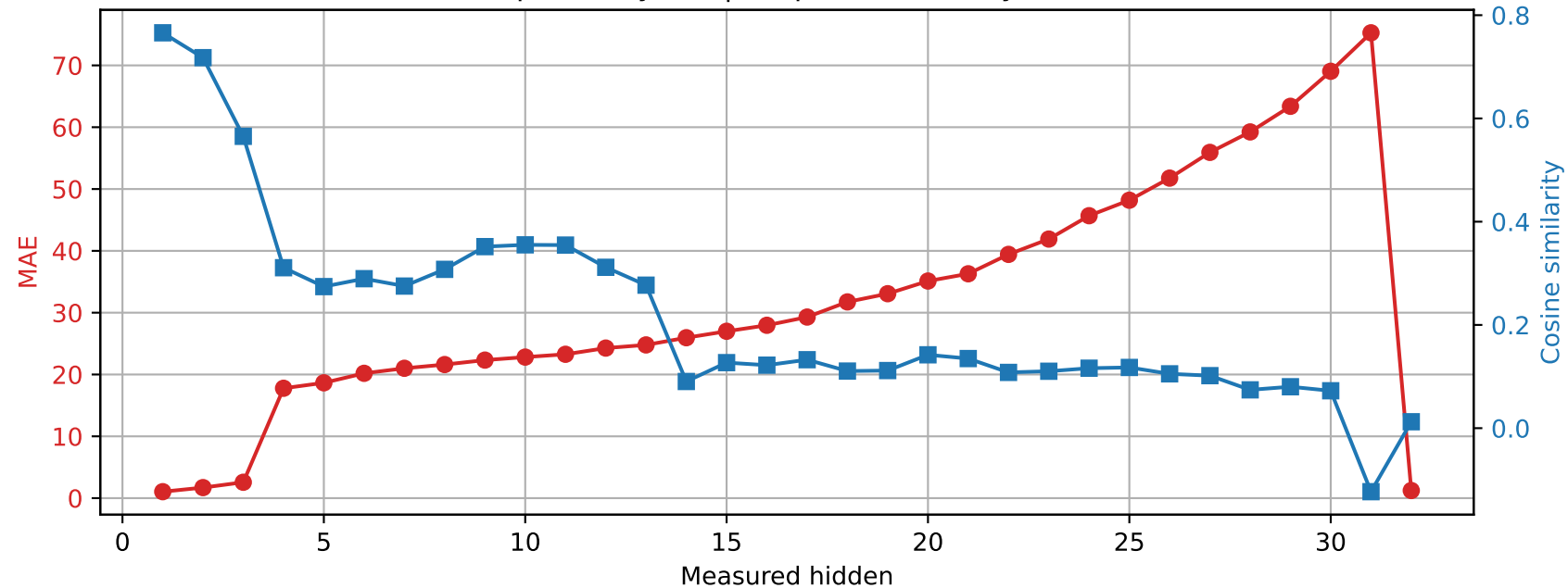
SmolLM2-360M | Prompt 0 Spared layer 7 | Unquantized vs hybrid
