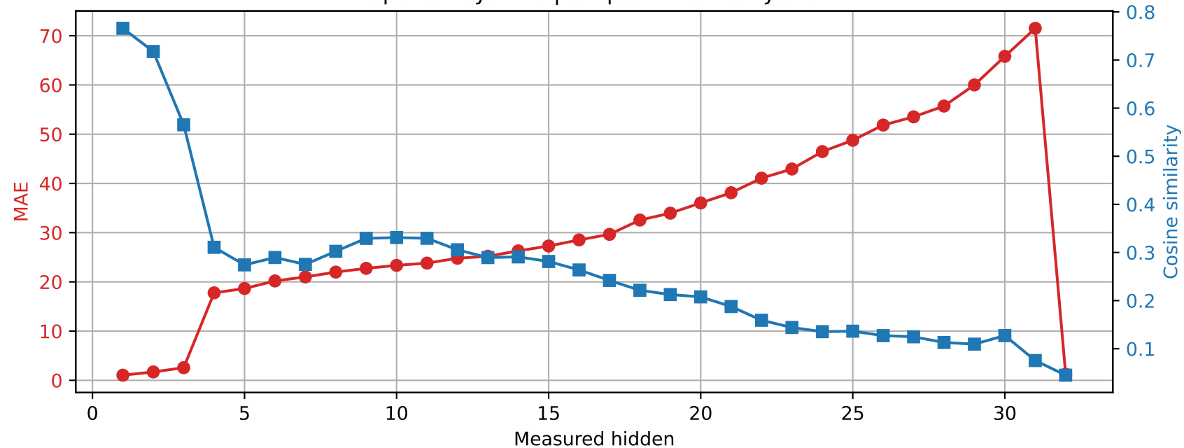
SmolLM2-360M | Prompt 0 Spared layer 26 | Unquantized vs hybrid
