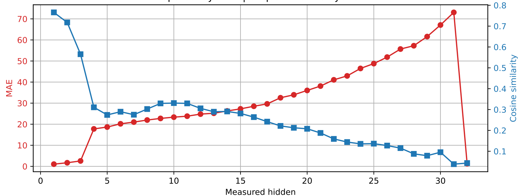
SmolLM2-360M | Prompt 0 Spared layer 27 | Unquantized vs hybrid
