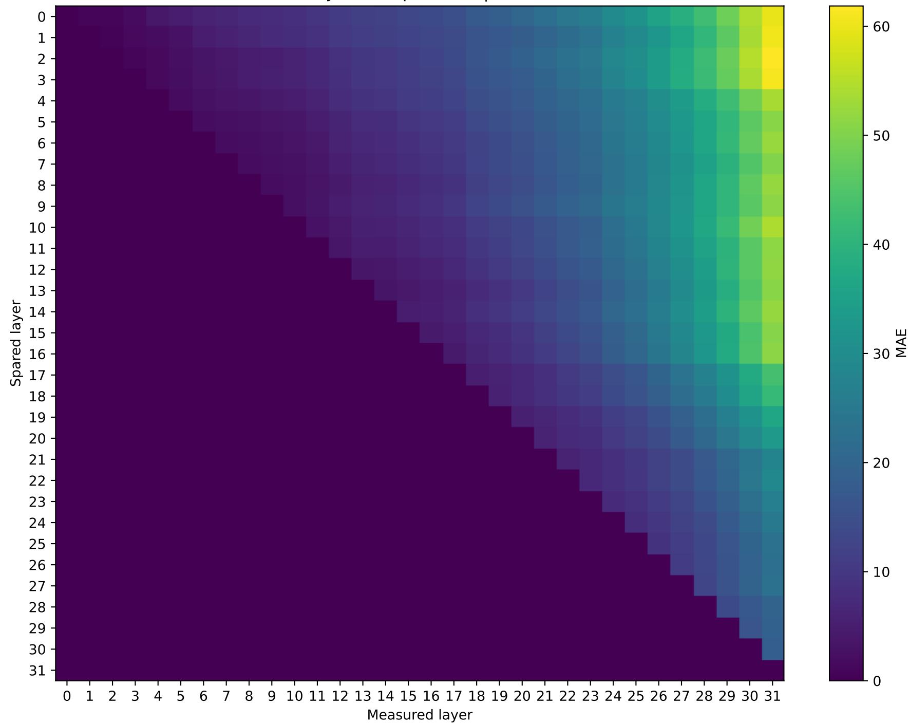
SmolLM2-360M | Prompt 1
