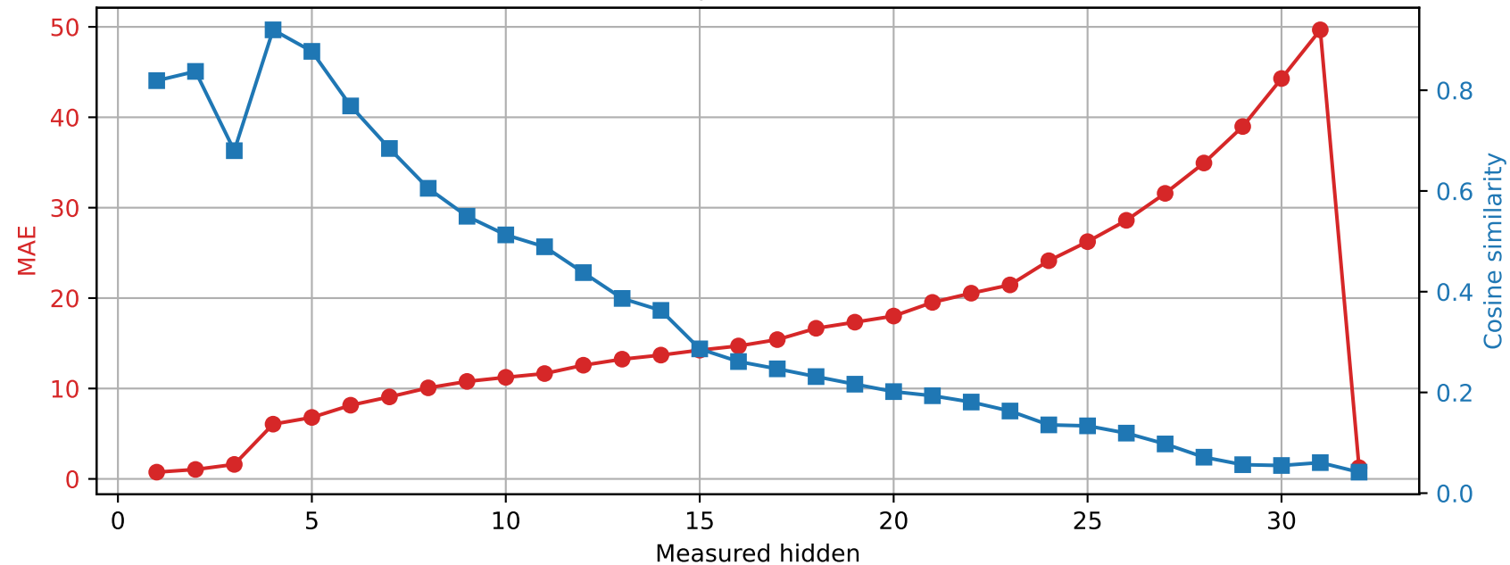
SmolLM2-360M | Prompt 1 Spared layer 1 | Unquantized vs hybrid
