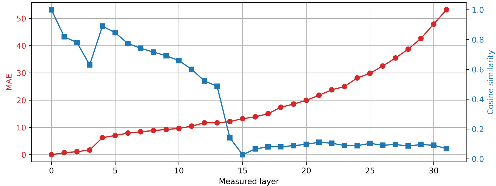
SmolLM2-360M | Prompt 1 Spared layer 12 | Hybrid vs unquantized
