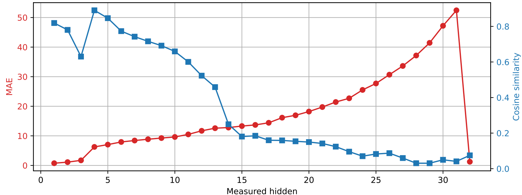
SmolLM2-360M | Prompt 1 Spared layer 13 | Unquantized vs hybrid
