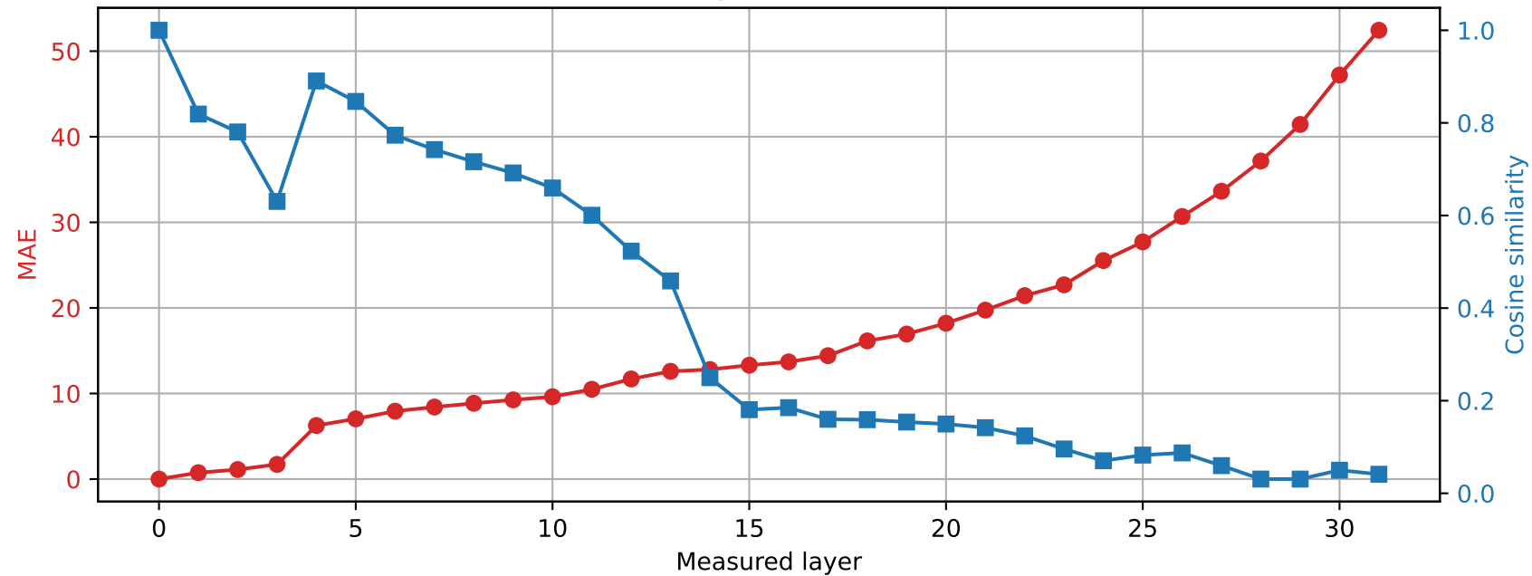
SmolLM2-360M | Prompt 1 Spared layer 13 | Hybrid vs unquantized
