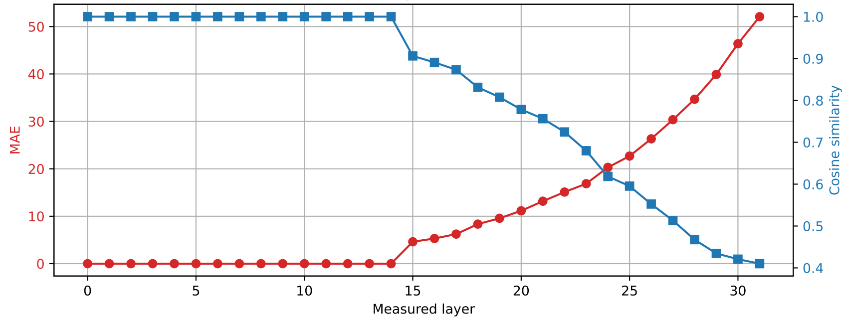
SmolLM2-360M | Prompt 1 Spared layer 14 | Hybrid vs quantized
