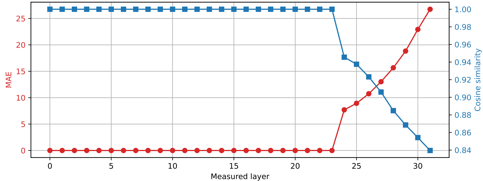
SmolLM2-360M | Prompt 1 Spared layer 23 | Hybrid vs quantized
