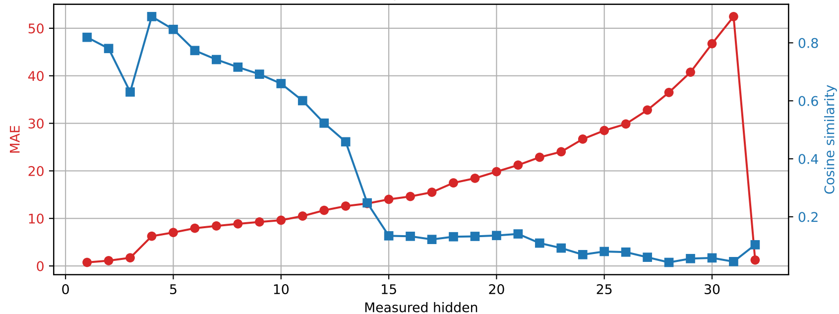
SmolLM2-360M | Prompt 1 Spared layer 25 | Unquantized vs hybrid
