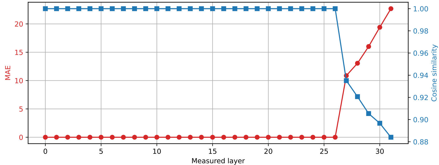
SmolLM2-360M | Prompt 1 Spared layer 26 | Hybrid vs quantized
