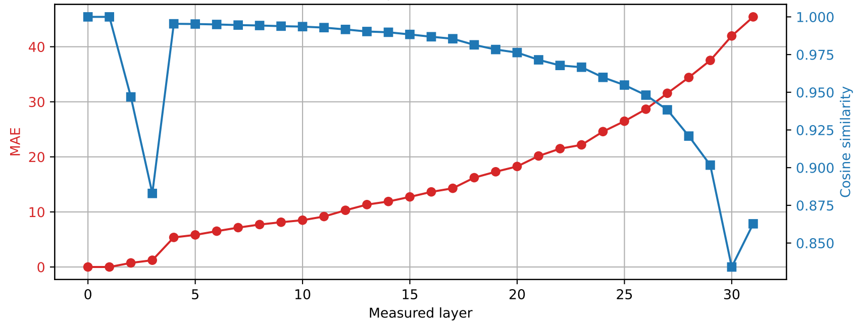
SmolLM2-360M | Prompt 2 Spared layer 0 | Hybrid vs unquantized
