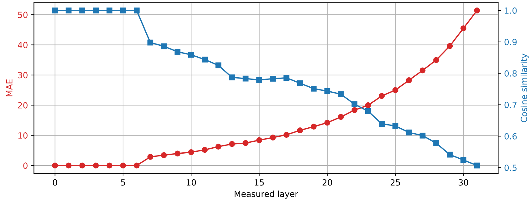
SmolLM2-360M | Prompt 2 Spared layer 6 | Hybrid vs quantized
