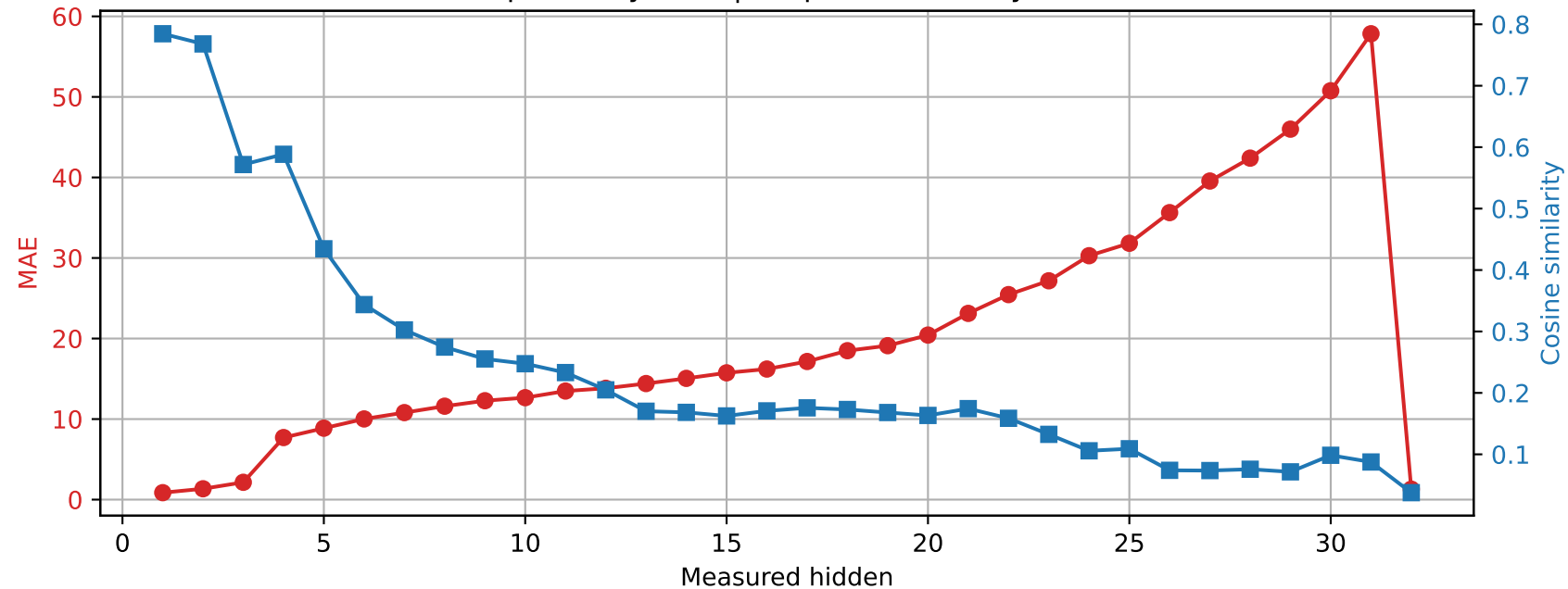
SmolLM2-360M | Prompt 2 Spared layer 11 | Unquantized vs hybrid
