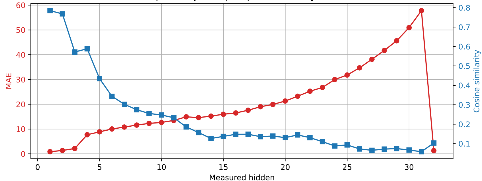
SmolLM2-360M | Prompt 2 Spared layer 12 | Unquantized vs hybrid
