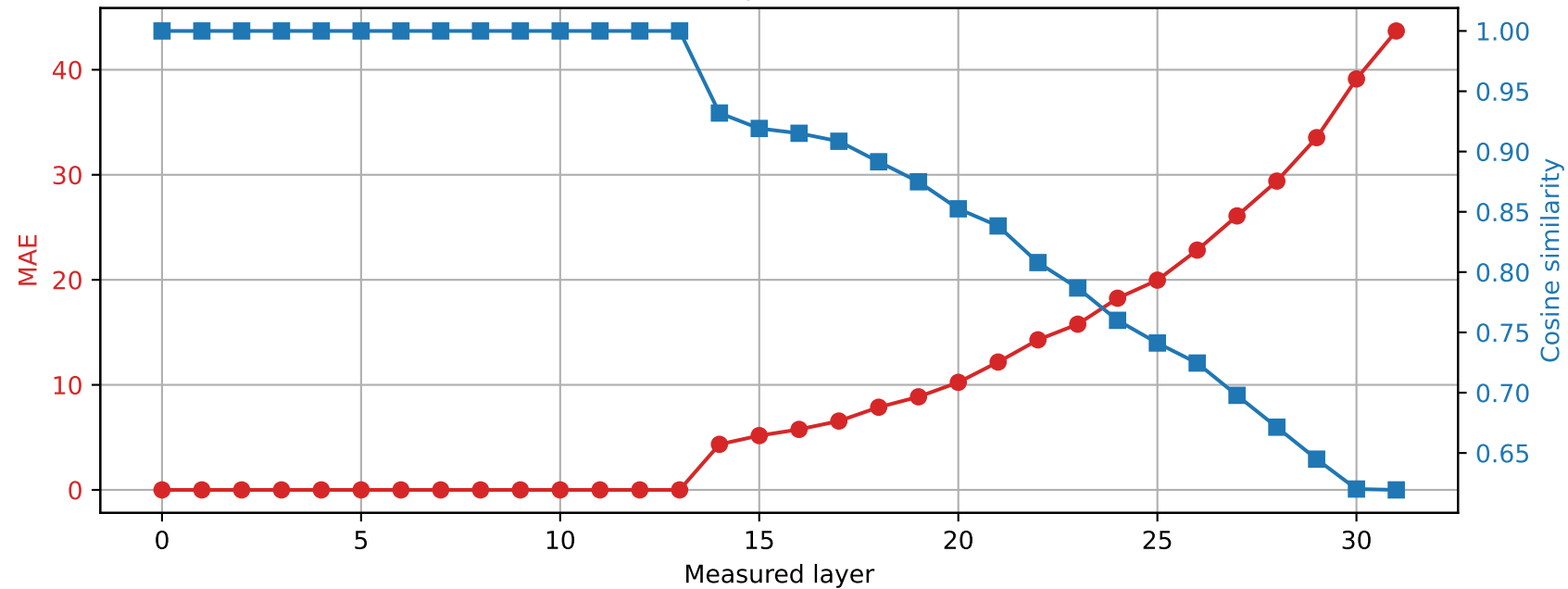
SmolLM2-360M | Prompt 2 Spared layer 13 | Hybrid vs quantized
