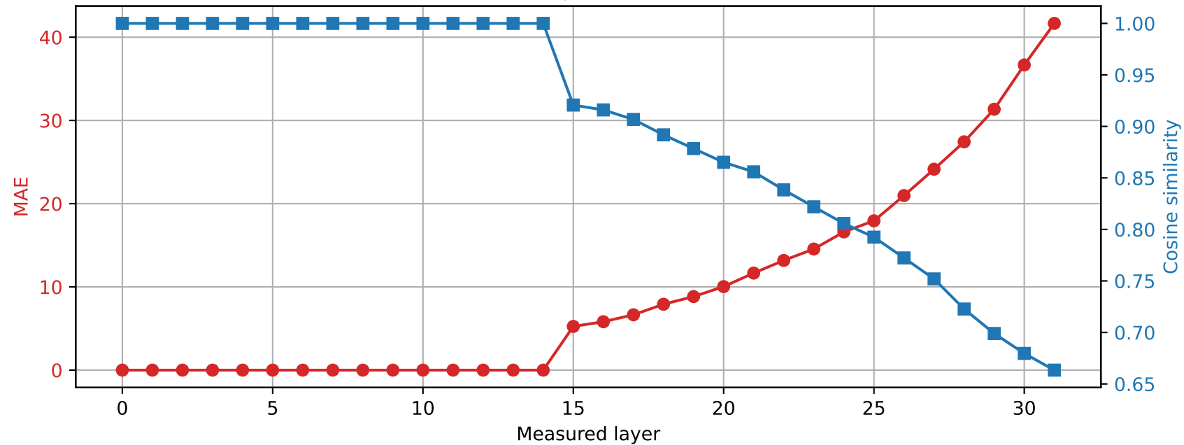
SmolLM2-360M | Prompt 2 Spared layer 14 | Hybrid vs quantized
