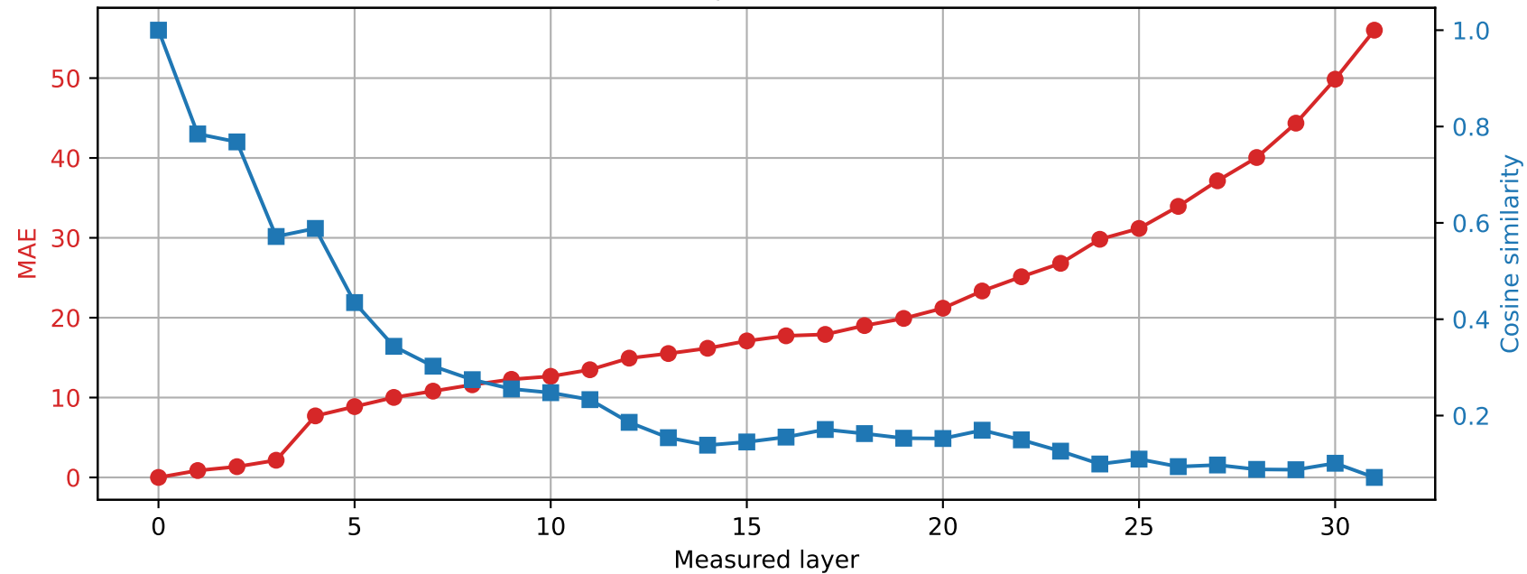
SmolLM2-360M | Prompt 2 Spared layer 16 | Hybrid vs unquantized
