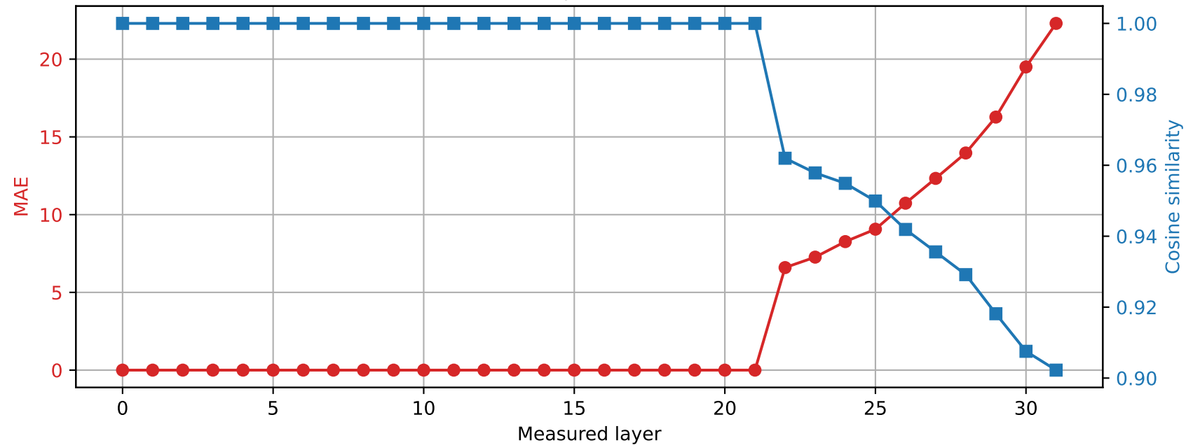
SmolLM2-360M | Prompt 2 Spared layer 21 | Hybrid vs quantized
