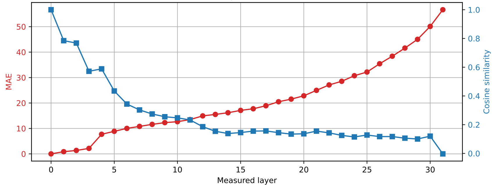
SmolLM2-360M | Prompt 2 Spared layer 23 | Hybrid vs unquantized
