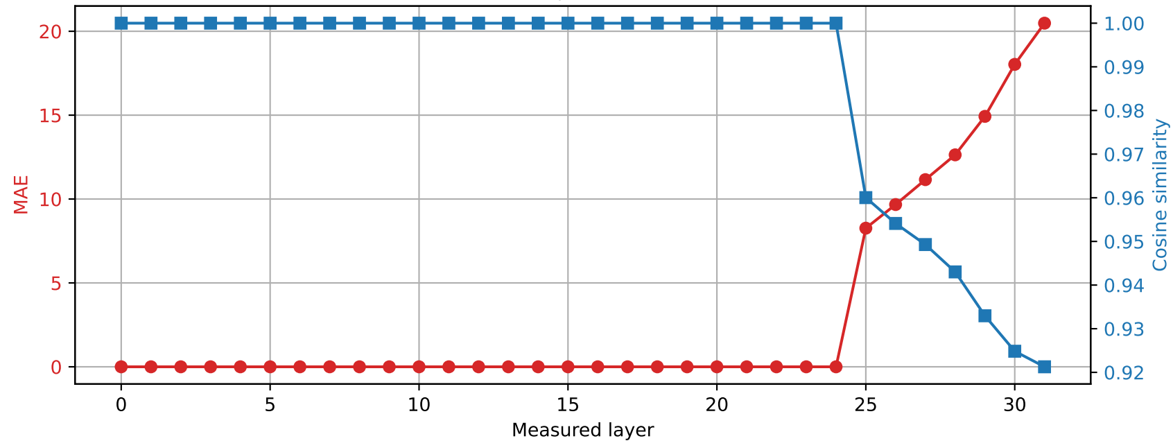
SmolLM2-360M | Prompt 2 Spared layer 24 | Hybrid vs quantized
