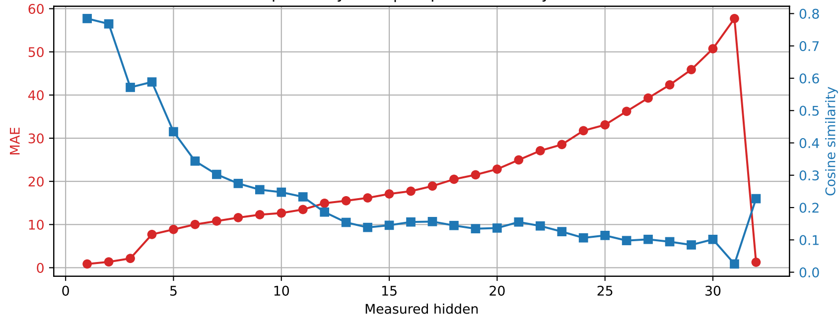
SmolLM2-360M | Prompt 2 Spared layer 31 | Unquantized vs hybrid
