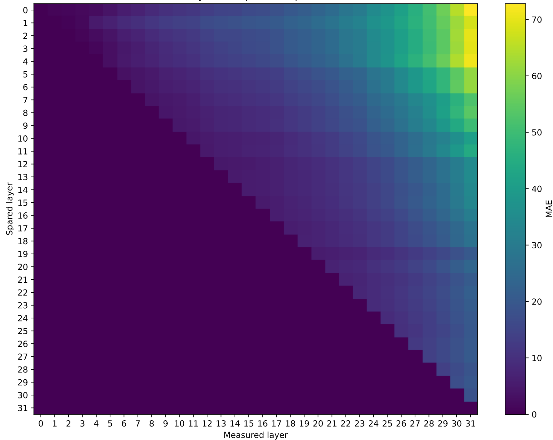
SmolLM2-360M | Prompt 3 Hybrid vs quantized | int4
