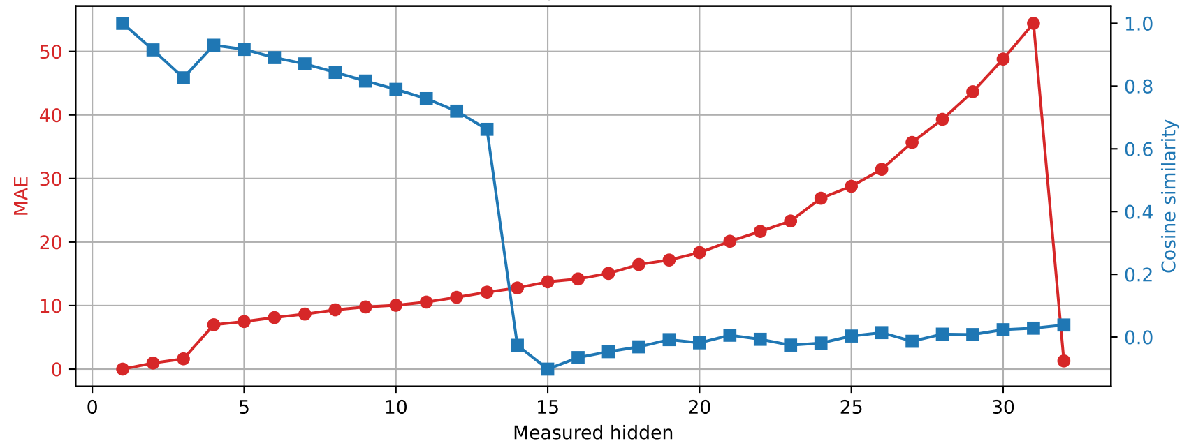
SmolLM2-360M | Prompt 3 Spared layer 0 | Unquantized vs hybrid
