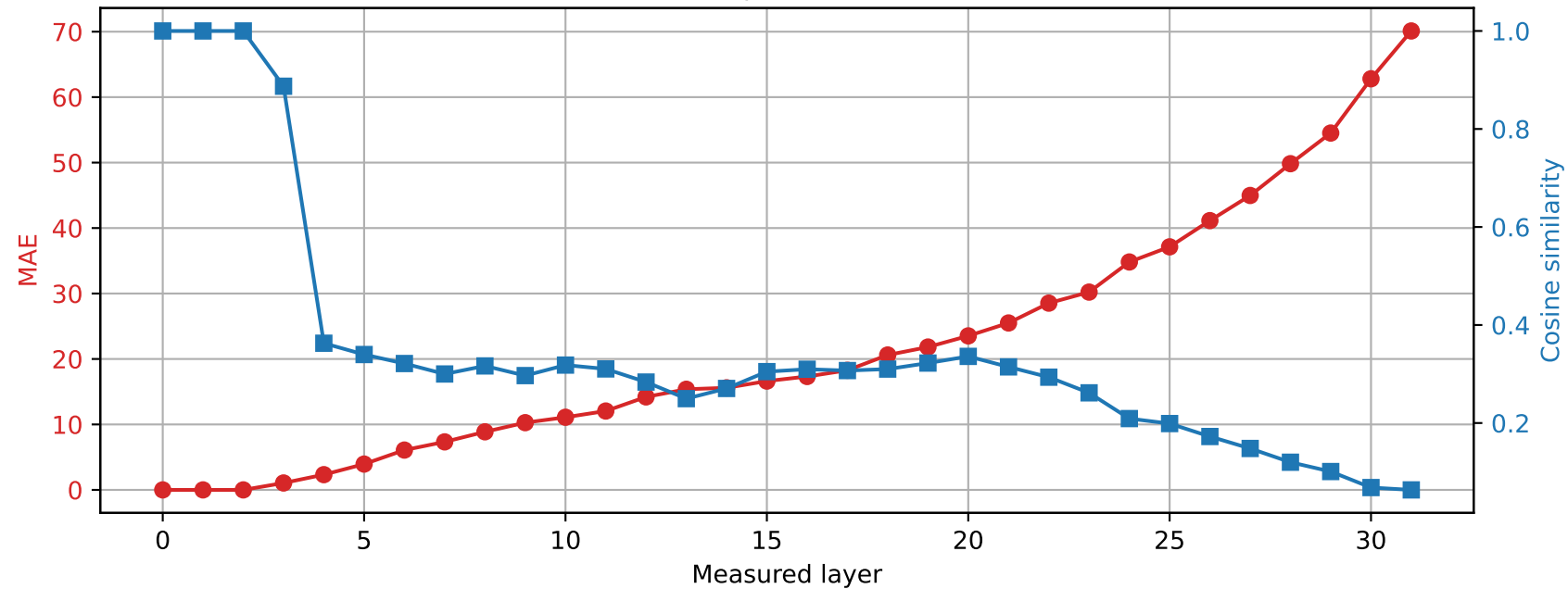
SmolLM2-360M | Prompt 3 Spared layer 2 | Hybrid vs quantized
