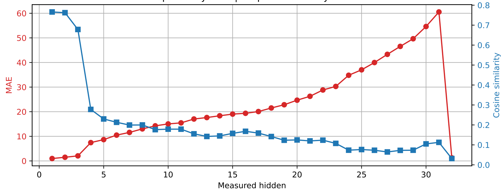
SmolLM2-360M | Prompt 3 Spared layer 10 | Unquantized vs hybrid
