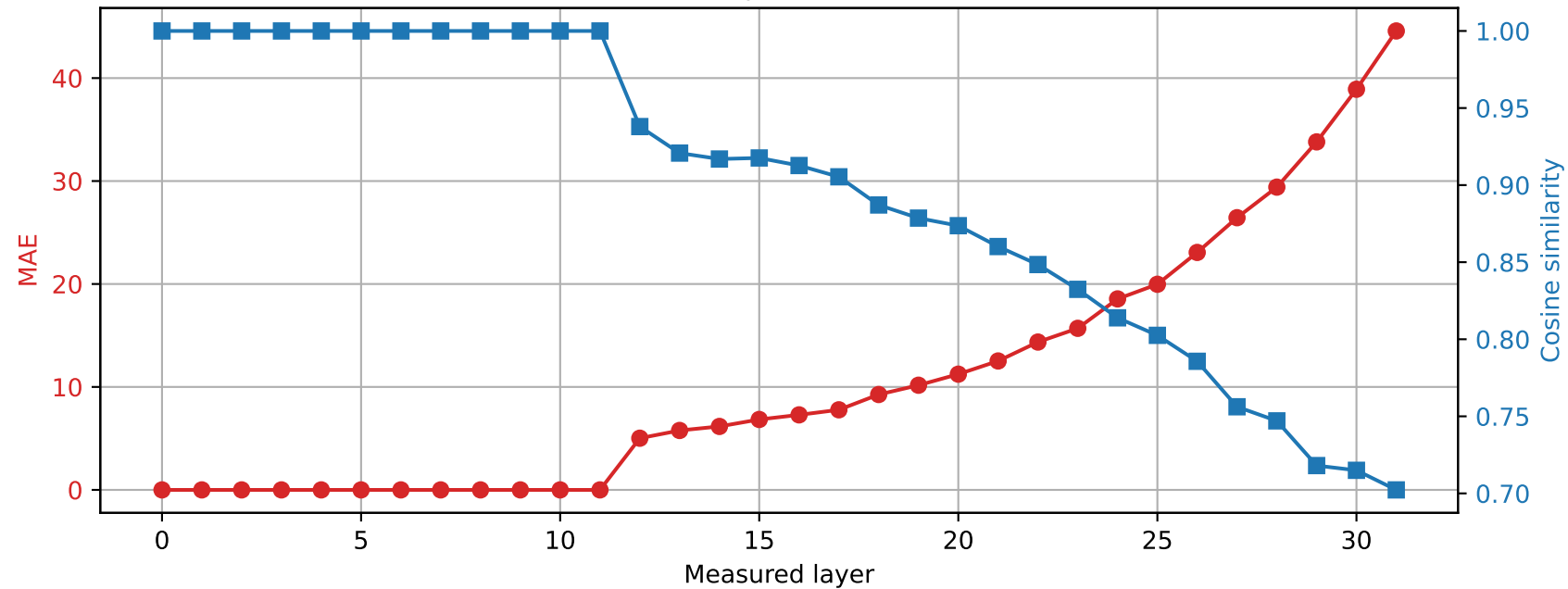
SmolLM2-360M | Prompt 3 Spared layer 11 | Hybrid vs quantized
