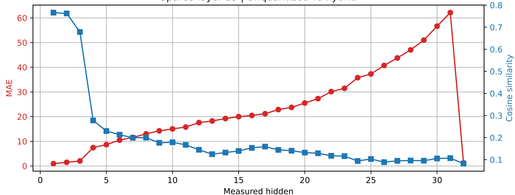
SmolLM2-360M | Prompt 3 Spared layer 13 | Unquantized vs hybrid
