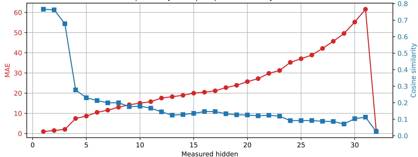
SmolLM2-360M | Prompt 3 Spared layer 25 | Unquantized vs hybrid
