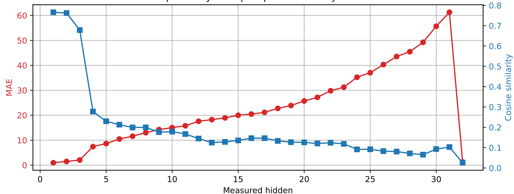
SmolLM2-360M | Prompt 3 Spared layer 27 | Unquantized vs hybrid
