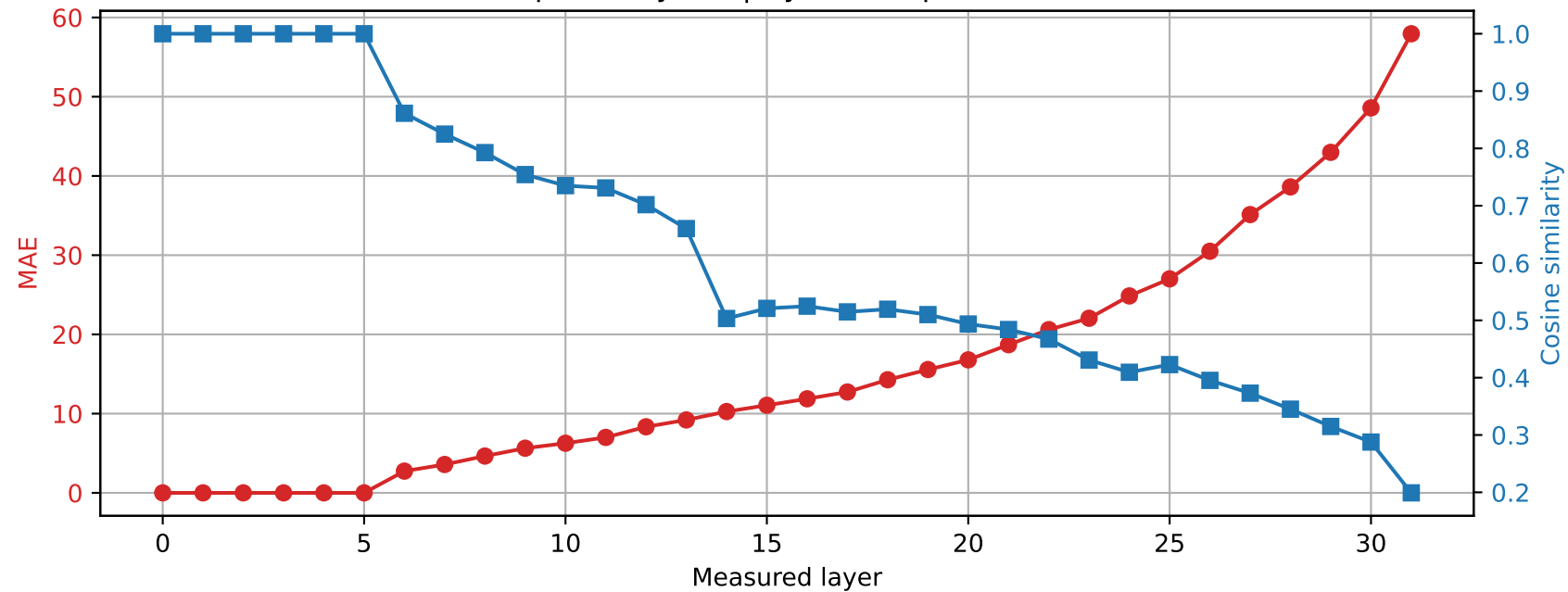
SmolLM2-360M | Prompt 4 Spared layer 5 | Hybrid vs quantized
