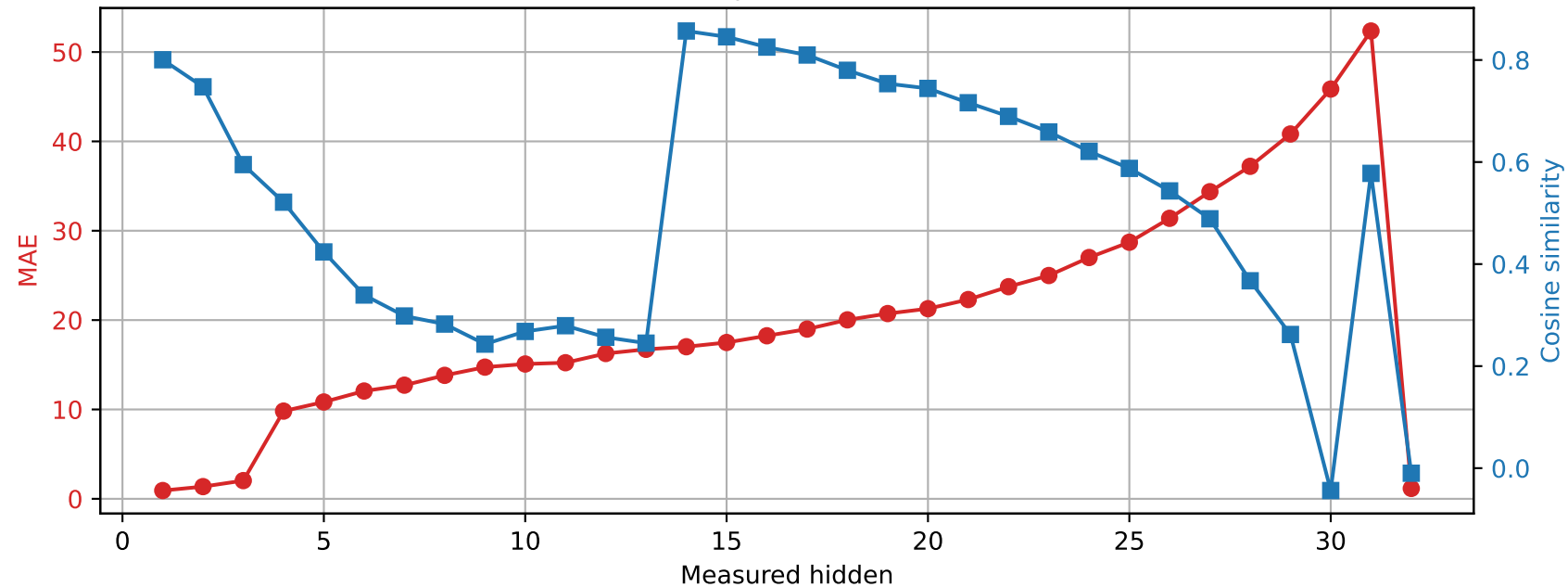
SmolLM2-360M | Prompt 4 Spared layer 10 | Unquantized vs hybrid
