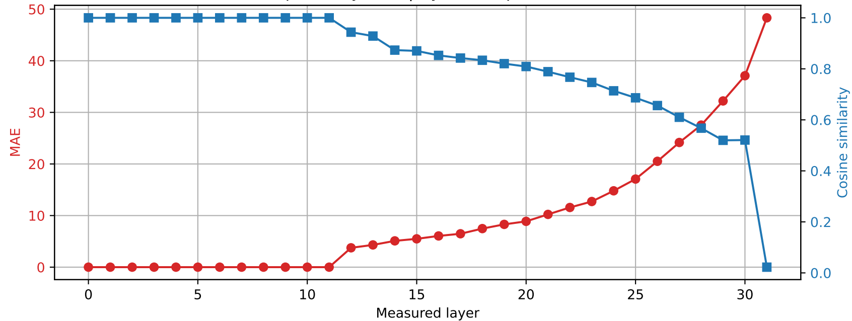
SmolLM2-360M | Prompt 4 Spared layer 11 | Hybrid vs quantized
