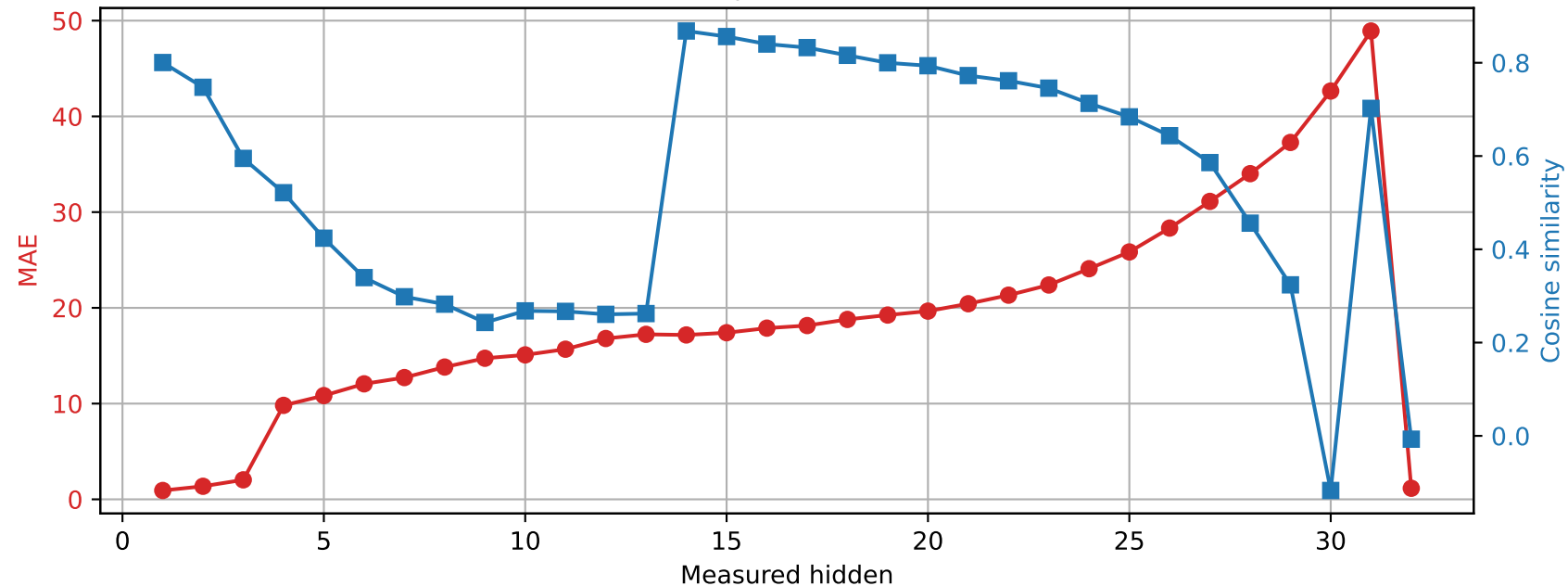
SmolLM2-360M | Prompt 4 Spared layer 13 | Unquantized vs hybrid
