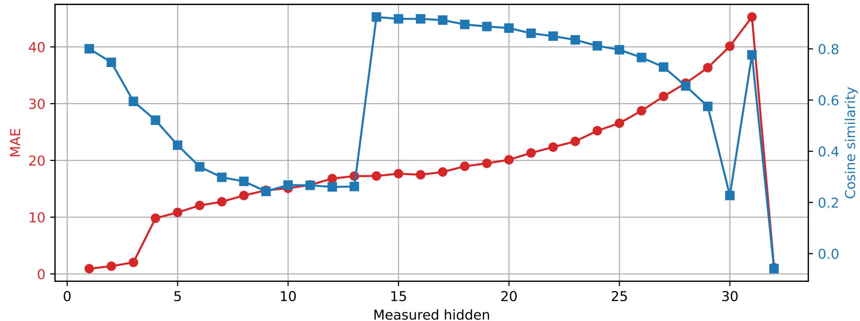
SmolLM2-360M | Prompt 4 Spared layer 15 | Unquantized vs hybrid
