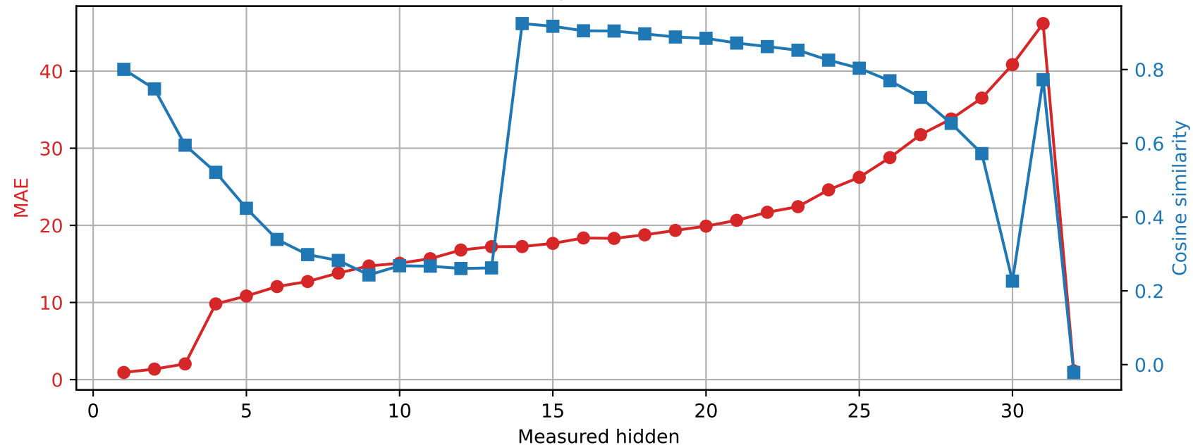
SmolLM2-360M | Prompt 4 Spared layer 16 | Unquantized vs hybrid
