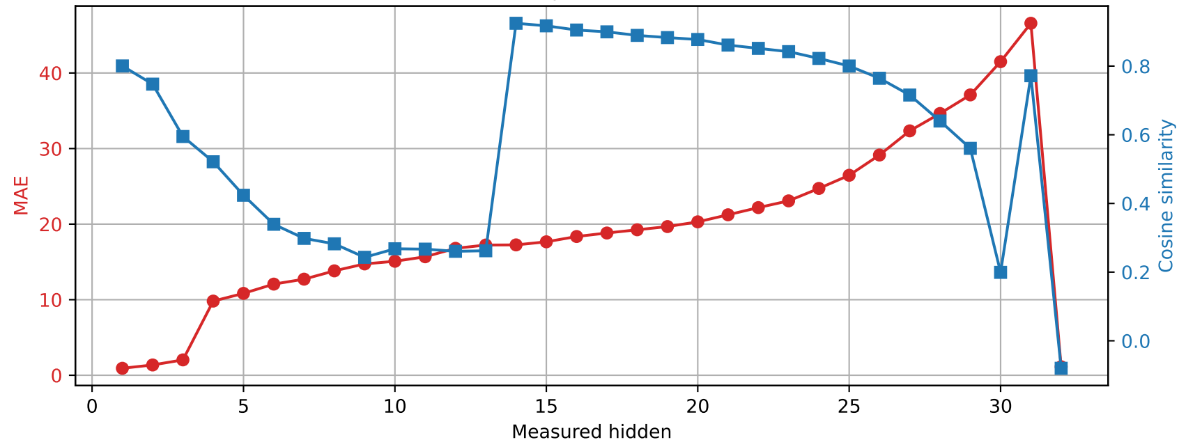
SmolLM2-360M | Prompt 4 Spared layer 17 | Unquantized vs hybrid
